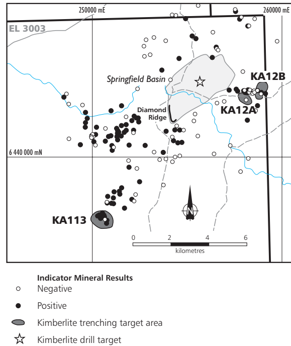
Figure 3 Springfield trenching targets.
