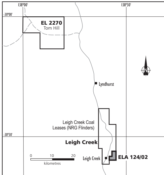
Figure 4 Leigh Creek exploration licence application.
