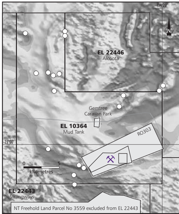
Figure 6 Strangways magnetic image and drill targets.
