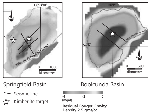
Figure 2 Gravity images with seismic lines and kimberlite targets.
